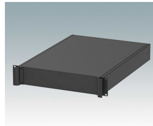
M6219279 COMBIMET 19" 2Ux610mm Aluminium Black RAL 9005 88.1x482.6x609.6mm
