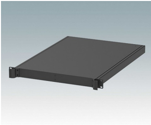
M6219179 COMBIMET 19" 1Ux610mm Aluminium Black RAL 9005 43.6x482.6x609.6mm
