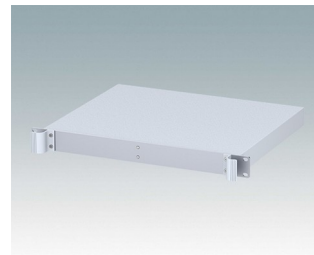
M6219125 COMBIMET 19" 1Ux365mm Solid Top Aluminium Light grey RAL 7035 43.6x482.6x365mm
