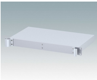
M6219115 COMBIMET 19" 1Ux265mm Solid Top Aluminium Light grey RAL 7035 43.6x482.6x265mm
