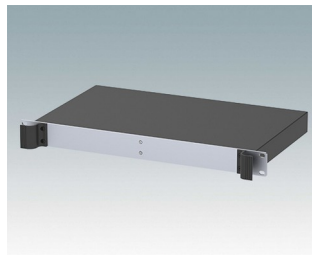
M6219119 COMBIMET 19" 1Ux265mm Solid Top Aluminium Black RAL 9005 43.6x482.6x265mm
